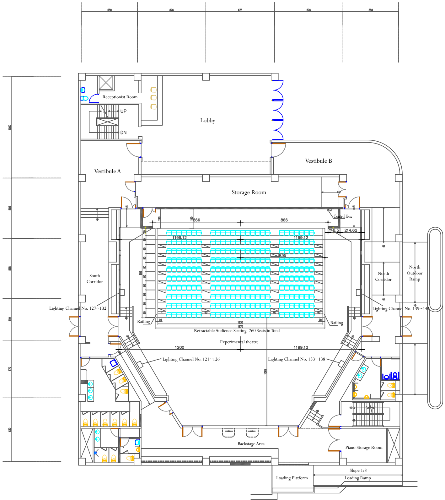
Appendix 1: International Hall (Native Theatre) 1st Floor Lighting Channel Plan
