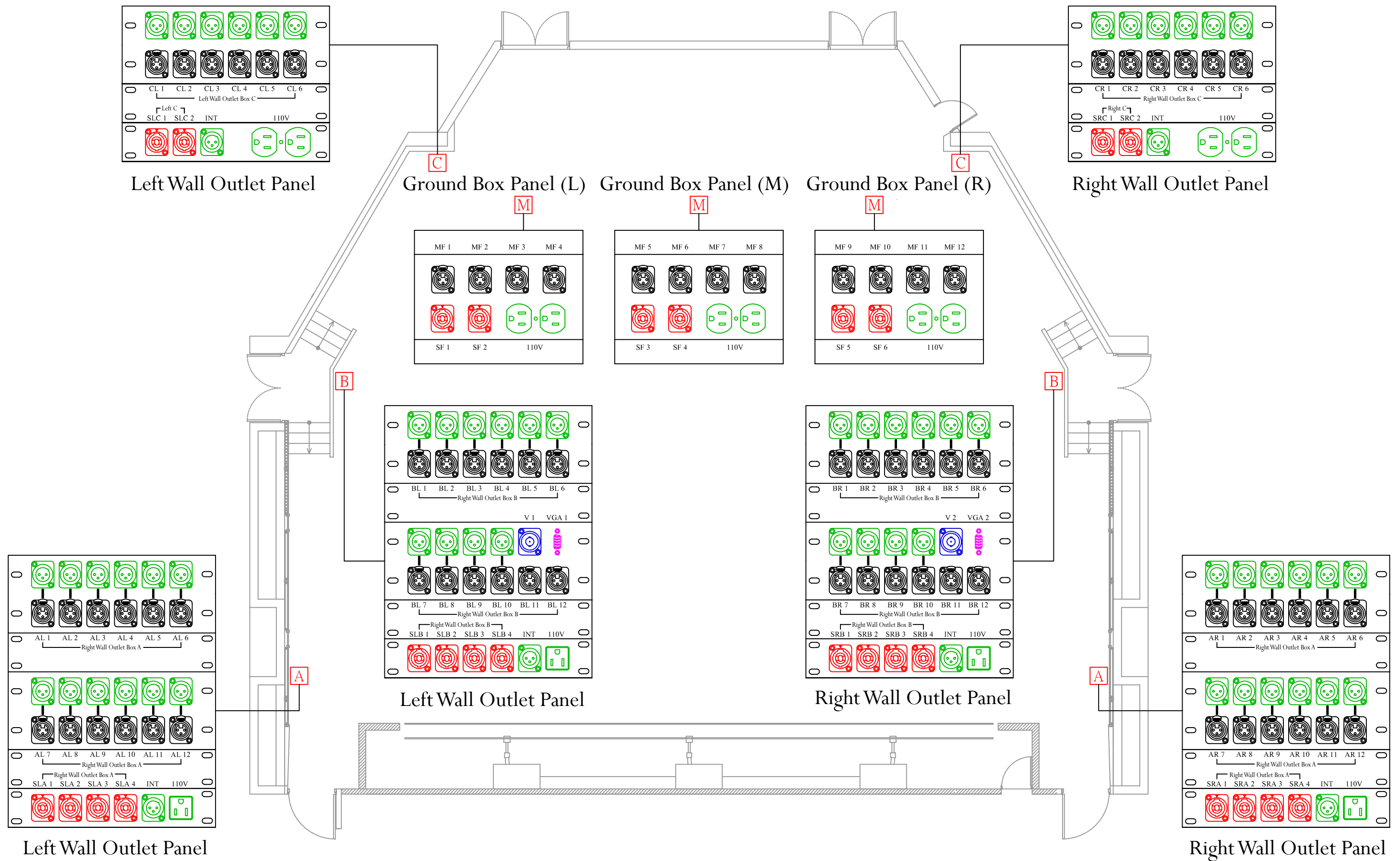
Appendix 3: International Hall (Native Theatre) 1st Floor Sound Panel Channel Plan
