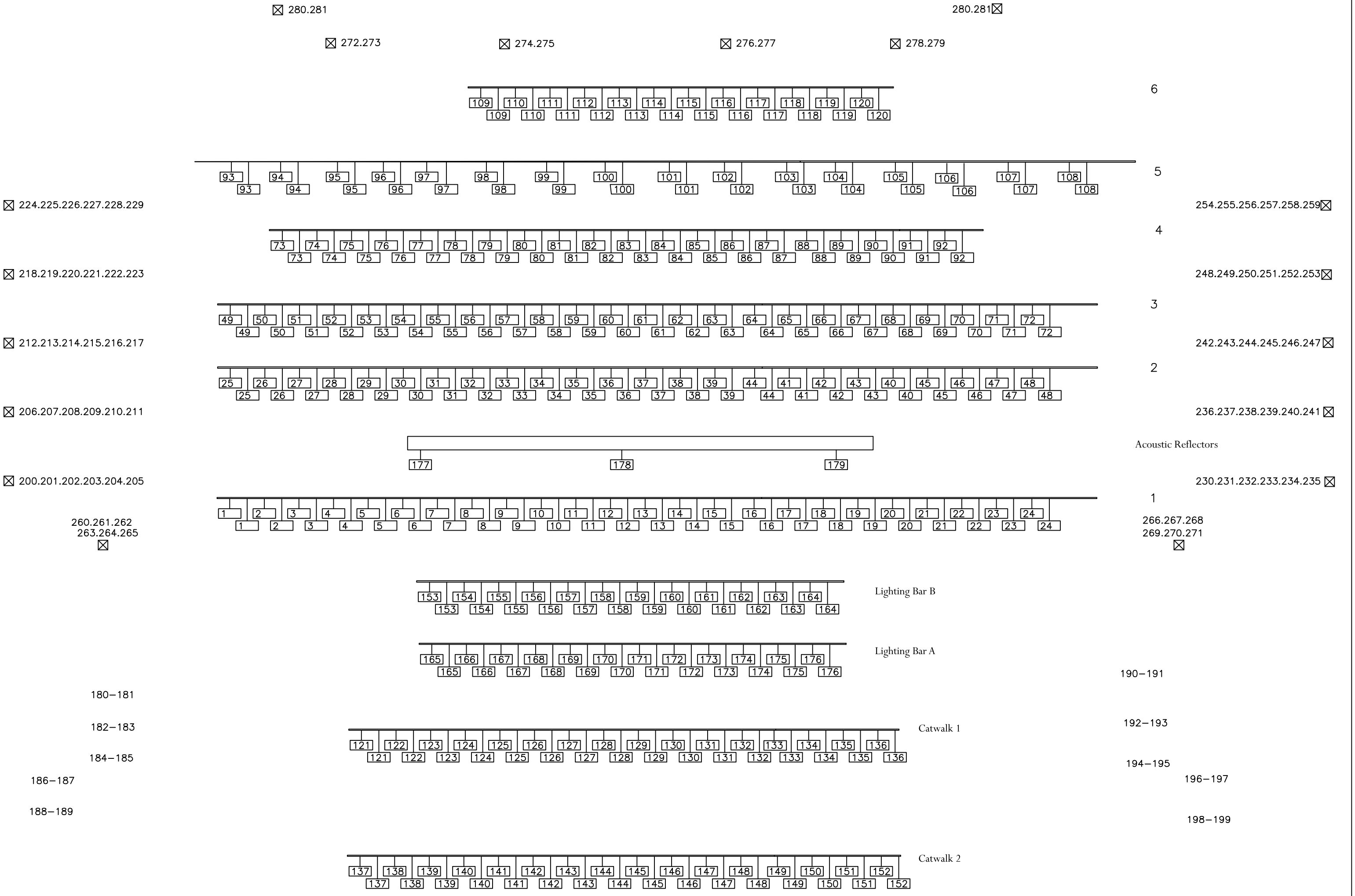
Lighting Channel Plan (Tainan Cultural Center Performance Hall)
