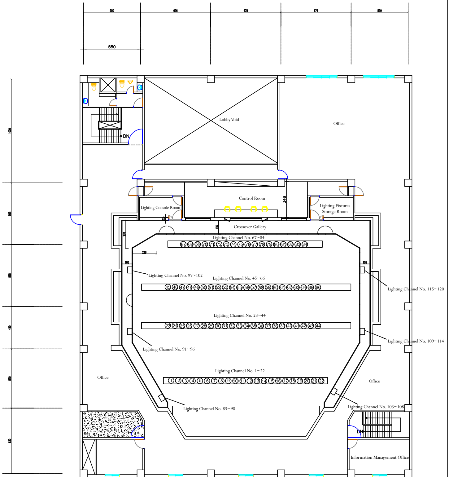
Appendix 2: International Hall (Native Theatre) 2nd Floor Lighting Channel Plan
